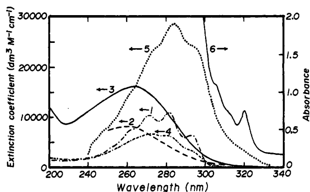
Figure 1. UV absorption spectra of (1) DHC, (2) previtamin, (3) vitamin D 3 , (4) lumisterol, and (5) tachesterol and (6) absorption spectrum of an aqueous solution of PSSS-VN ( c = 1 \text{ g dm}^{-3} , l = 1 \text{ cm} ) in a near-UV region.
