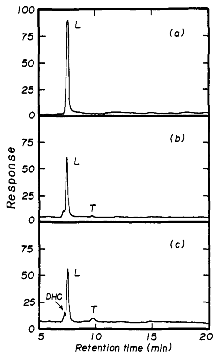
Figure 6. HPLC traces for lumisterol irradiated in the presence of naphthalene at 313 nm for various periods of time: (a) 0 min, (b) 15 min, and (c) 30 min.
