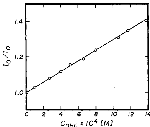
Figure 4. Stern–Volmer plot of the ratio of naphthalene fluorescence intensities ( I_0/I_Q ) in the absence ( I_0 ) and presence of quencher ( I_Q ) versus concentration of DHC in THF solution.
