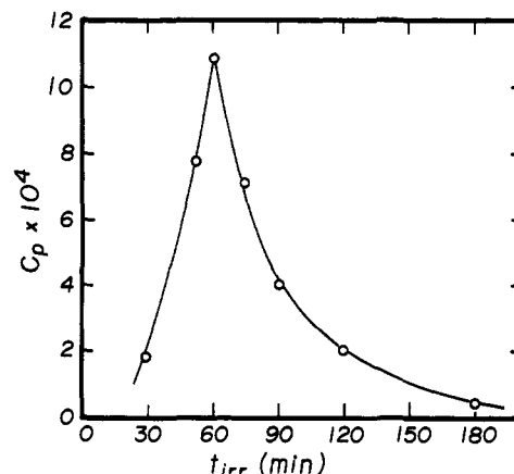
Figure 3. Dependence of the concentration of previtamin formed in a photozyme on the time of exposure to solar light ( c_{\text{pol}} = 1 \text{ g dm}^{-3} , c_{\text{DHC}} = 1.7 \times 10^{-4} M).
