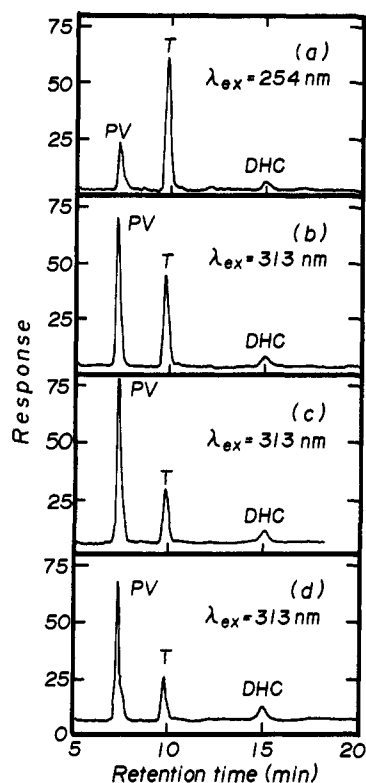
Figure 7. HPLC traces for DHC in cyclohexane irradiated for 120 min at (a) 254 nm and for mixtures obtained following the first-step naphthalene-sensitized reaction induced by irradiation at 313 nm for different periods of time: (b) 5 min, (c) 15 min, and (d) 30 min.
