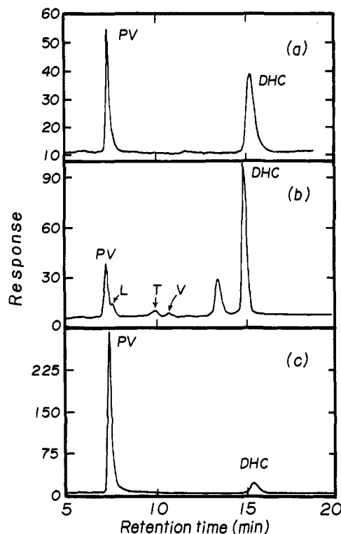
Figure 2. HPLC traces for the reaction mixtures obtained (a) after 90 min of solar irradiation of an aqueous solution of PSSS-VN containing solubilized DHC, (b) for DHC in cyclohexane solution irradiated 90 min with solar light, and (c) after 30 min of irradiation of an aqueous solution of PSSS-VN containing solubilized DHC ( c_{\text{DHC}} = 1.7 \times 10^{-4} M) with light at 313 nm.
