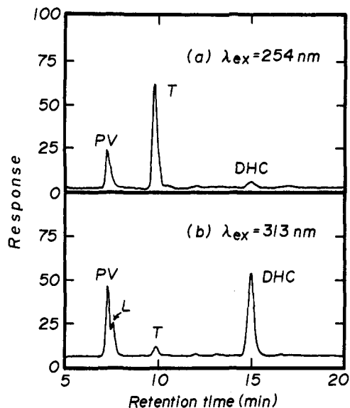
Figure 5. HPLC traces for DHC in cyclohexane solution irradiated for 120 min at (a) 254 and (b) 313 nm.
